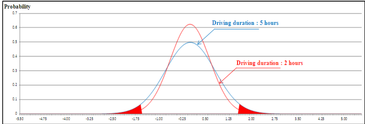
Figure 4. Deceleration and acceleration distribution of driver 12
